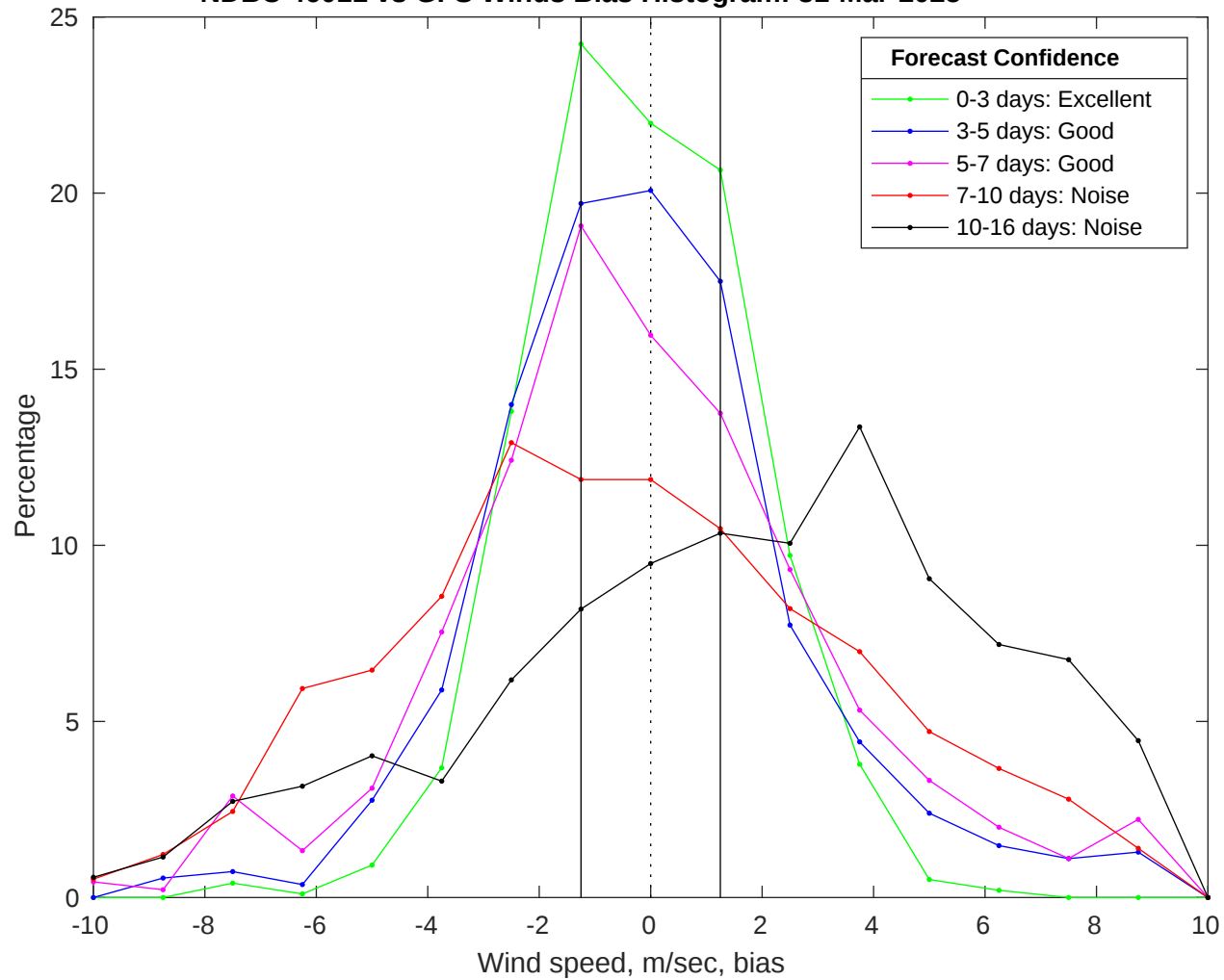
NDBC 46011 vs GFS Winds Bias Histogram: 31-Mar-2025
