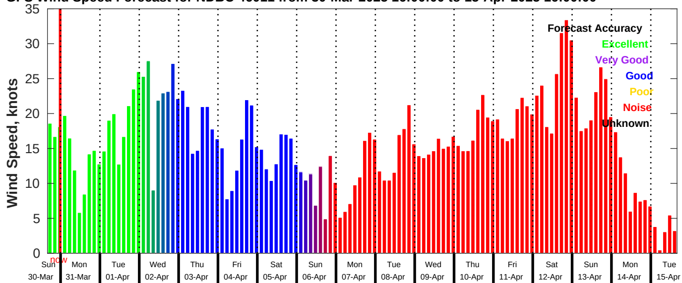
GFS Wind Speed Forecast for NDBC 46011 from 30-Mar-2025 16:00:00 to 15-Apr-2025 16:00:00
