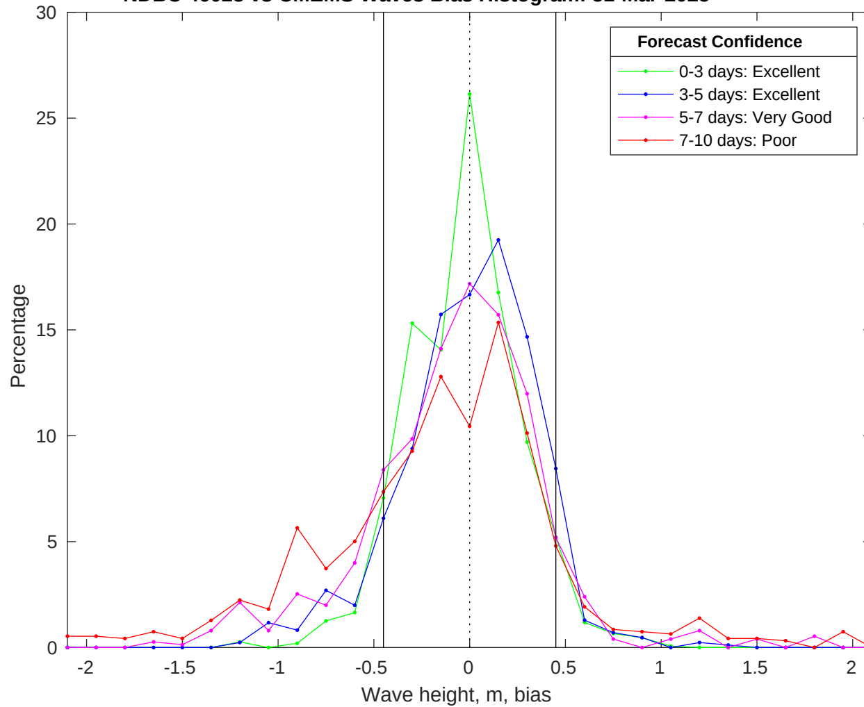
NDBC 46028 vs CMEMS Waves Bias Histogram: 31-Mar-2025
