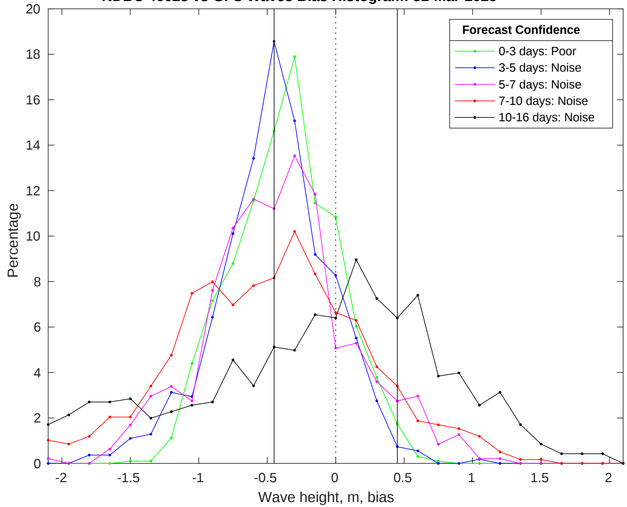
NDBC 46028 vs GFS Waves Bias Histogram: 31-Mar-2025
