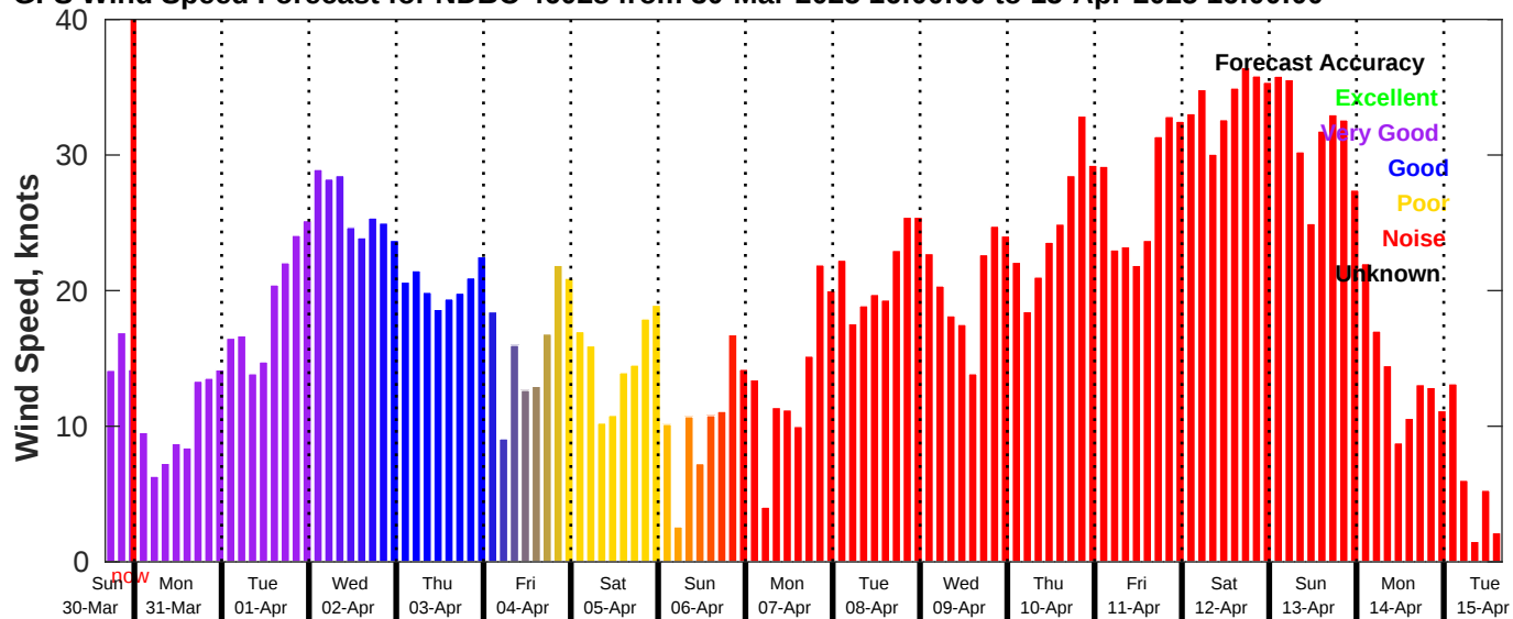
GFS Wind Speed Forecast for NDBC 46028 from 30-Mar-2025 16:00:00 to 15-Apr-2025 16:00:00
