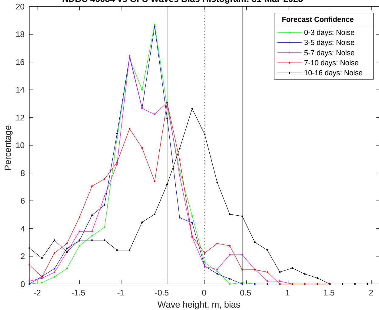
NDBC 46054 vs GFS Waves Bias Histogram: 31-Mar-2025
