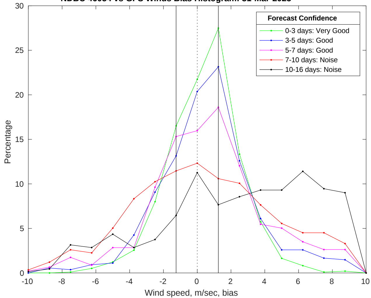
NDBC 46054 vs GFS Winds Bias Histogram: 31-Mar-2025
