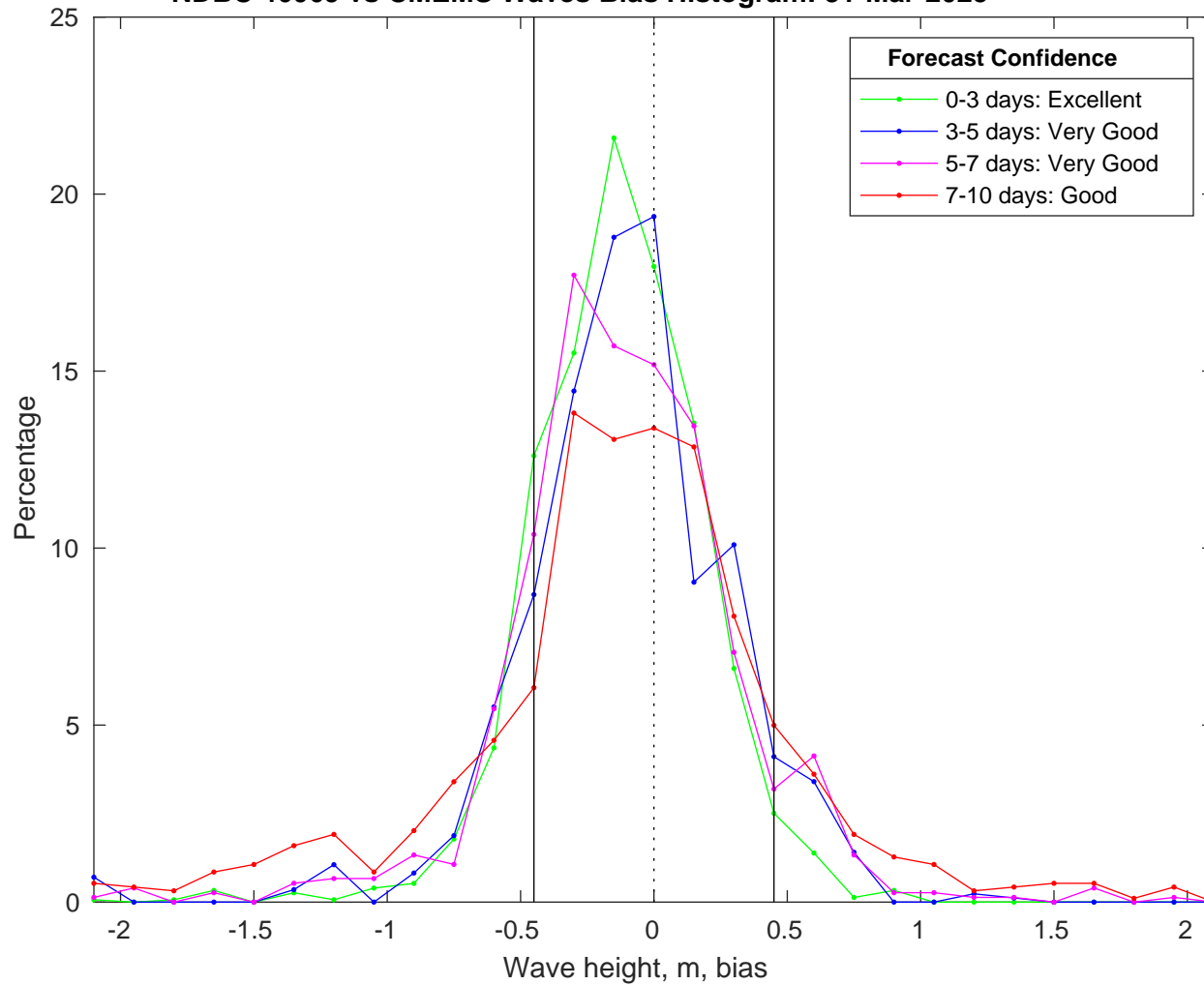
NDBC 46069 vs CMEMS Waves Bias Histogram: 31-Mar-2025
