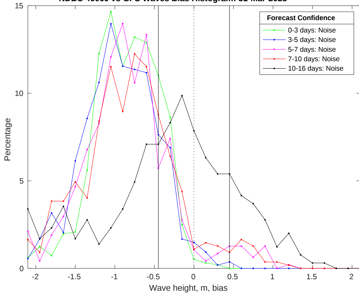
NDBC 46069 vs GFS Waves Bias Histogram: 31-Mar-2025
