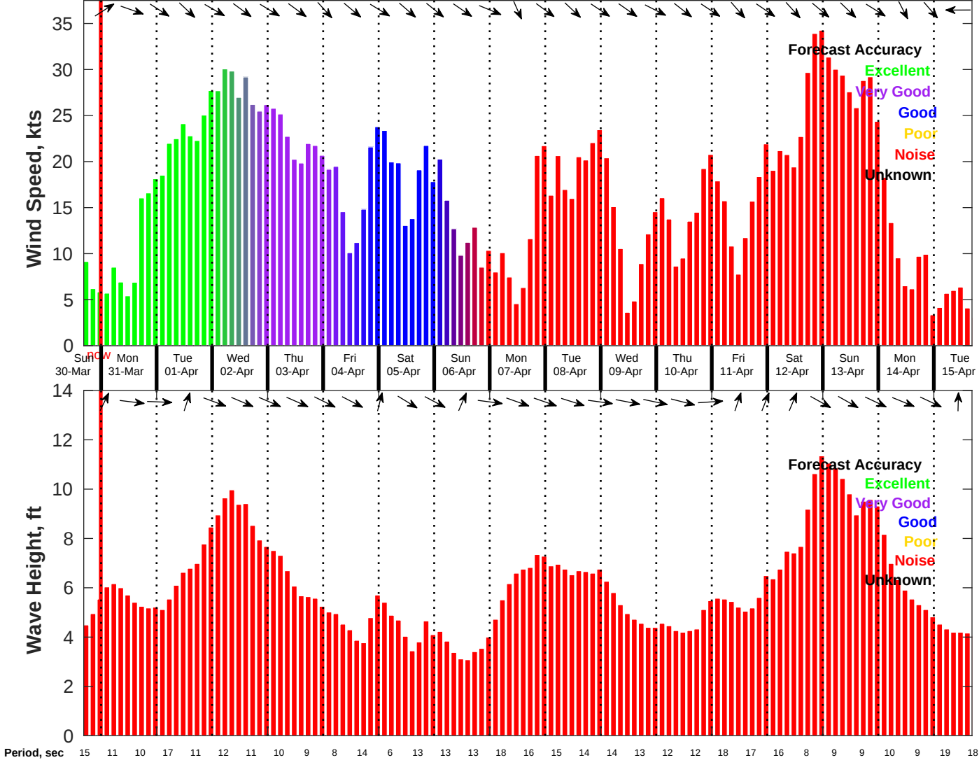
Wind & Wave Forecast for NDBC 46069 from 30-Mar-2025 16:00:00 to 15-Apr-2025 16:00:00
