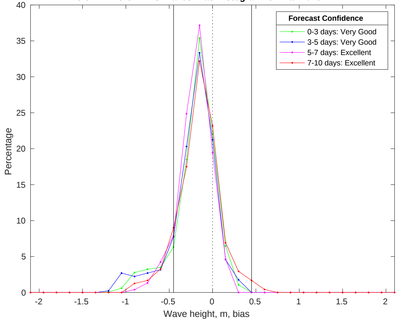
NDBC 52211 vs CMEMS Waves Bias Histogram: 31-Mar-2025
