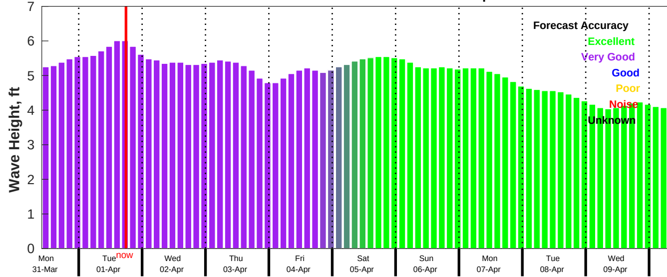
CMEMS Wave Forecast for NDBC 52211 from 30-Mar-2025 10:00:00 to 09-Apr-2025 10:00:00
