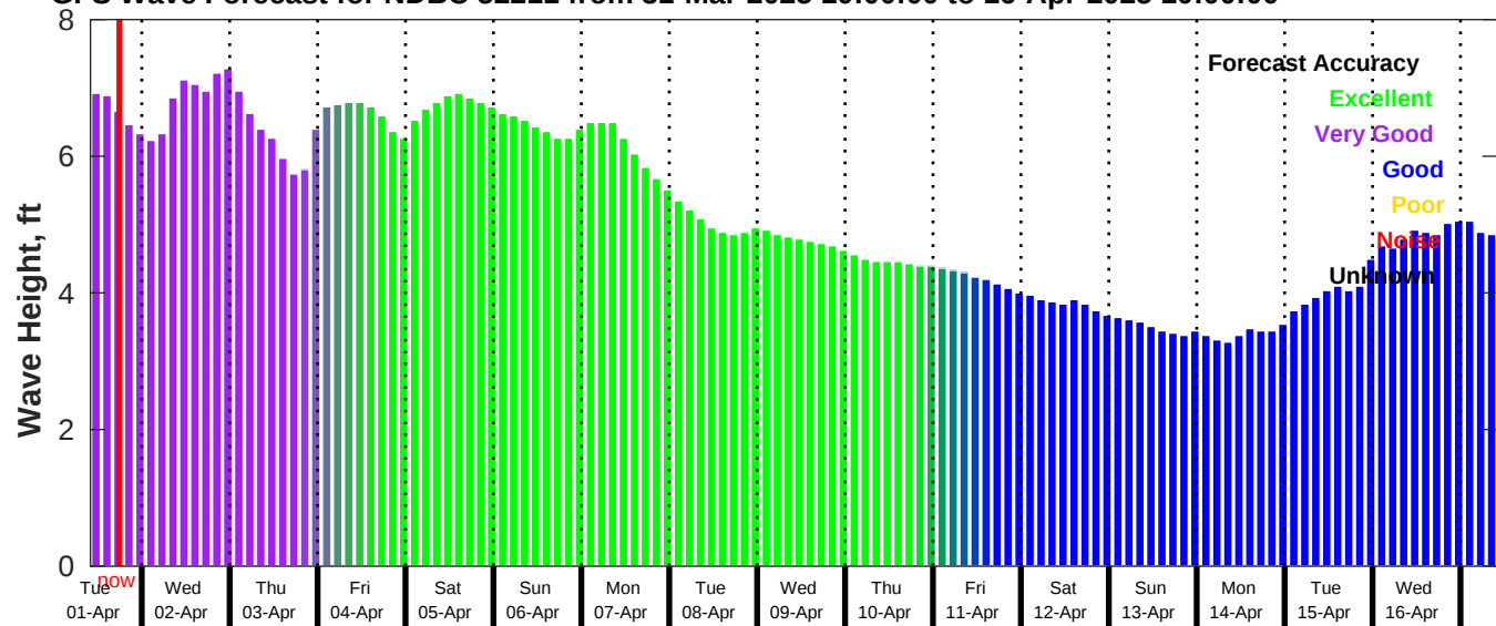
GFS Wave Forecast for NDBC 52211 from 31-Mar-2025 10:00:00 to 16-Apr-2025 10:00:00
