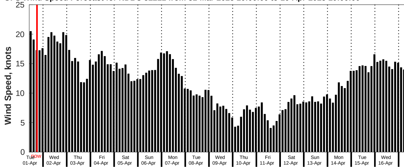
GFS Wind Speed Forecast for NDBC 52211 from 31-Mar-2025 10:00:00 to 16-Apr-2025 10:00:00
