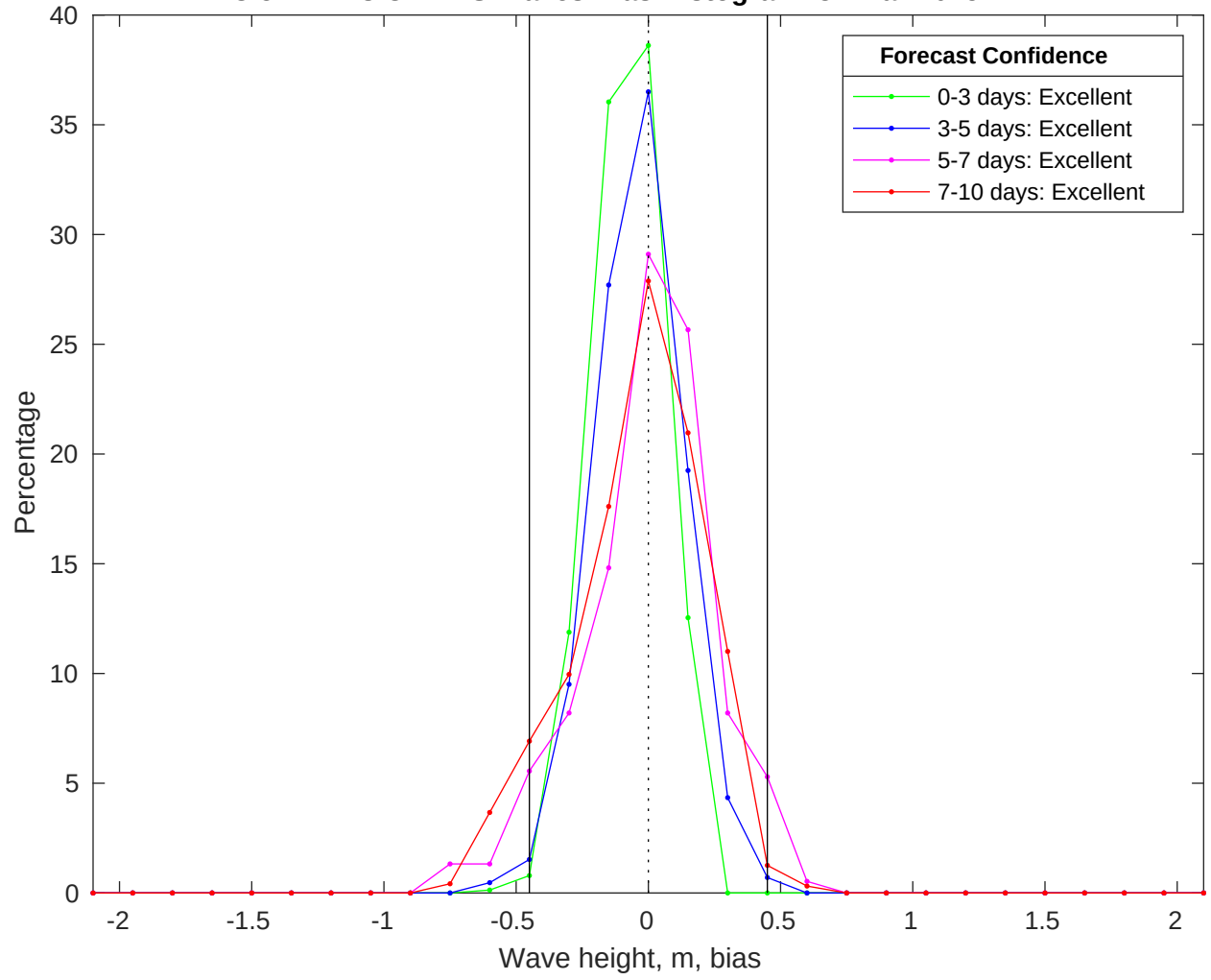
NDBC 52212 vs CMEMS Waves Bias Histogram: 31-Mar-2025
