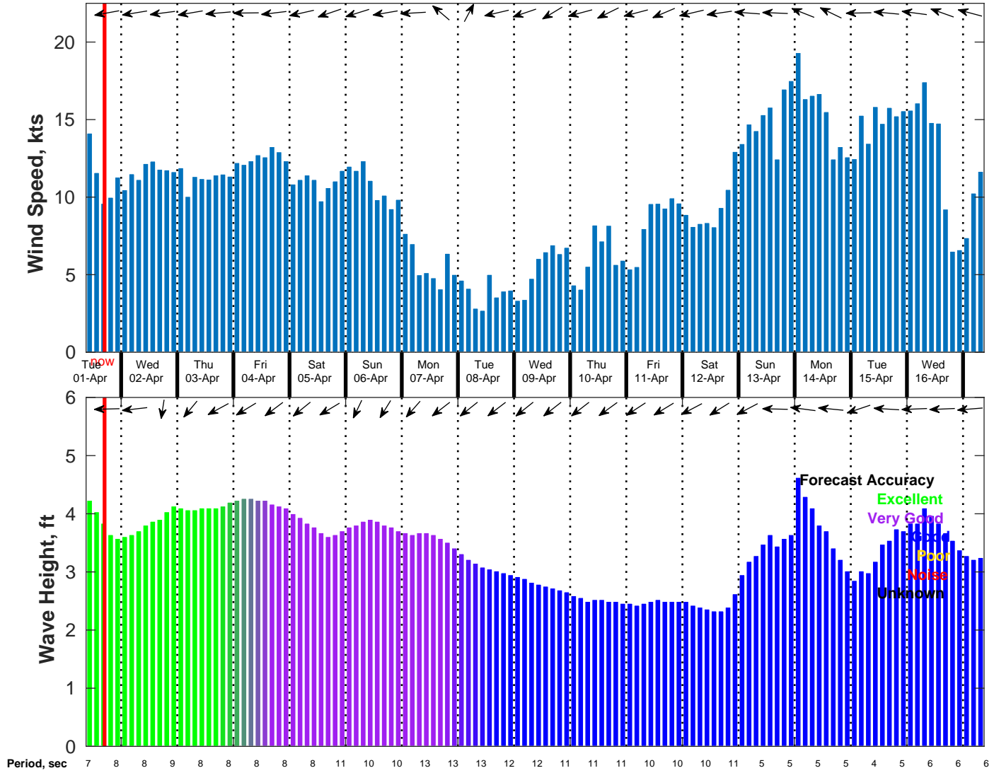
Wind & Wave Forecast for NDBC 52212 from 31-Mar-2025 09:00:00 to 16-Apr-2025 09:00:00
