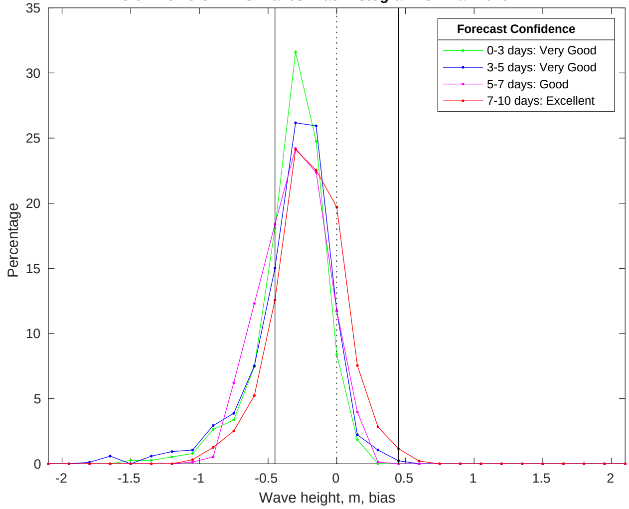
NDBC 52213 vs CMEMS Waves Bias Histogram: 31-Mar-2025
