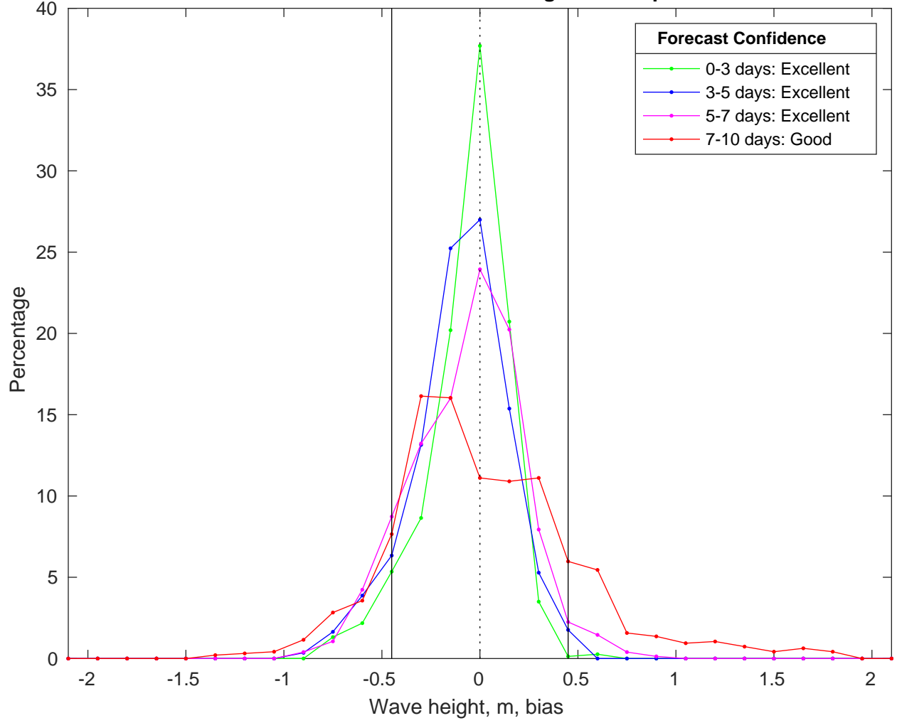
NDBC 41004 vs CMEMS Waves Bias Histogram: 01-Apr-2025
