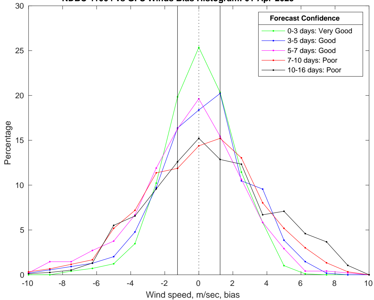
NDBC 41004 vs GFS Winds Bias Histogram: 01-Apr-2025
