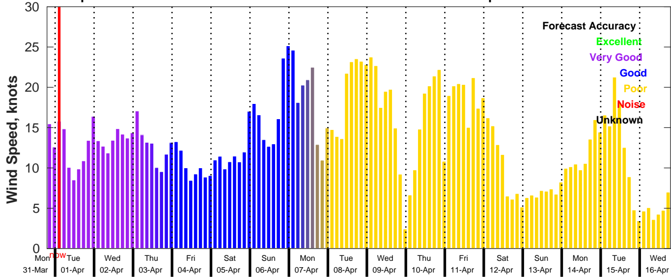
GFS Wind Speed Forecast for NDBC 41004 from 31-Mar-2025 19:00:00 to 16-Apr-2025 19:00:00
