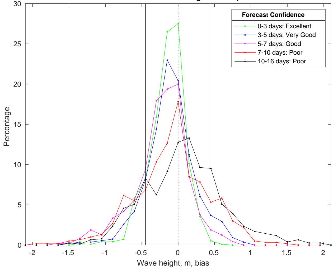
NDBC 41013 vs GFS Waves Bias Histogram: 01-Apr-2025
