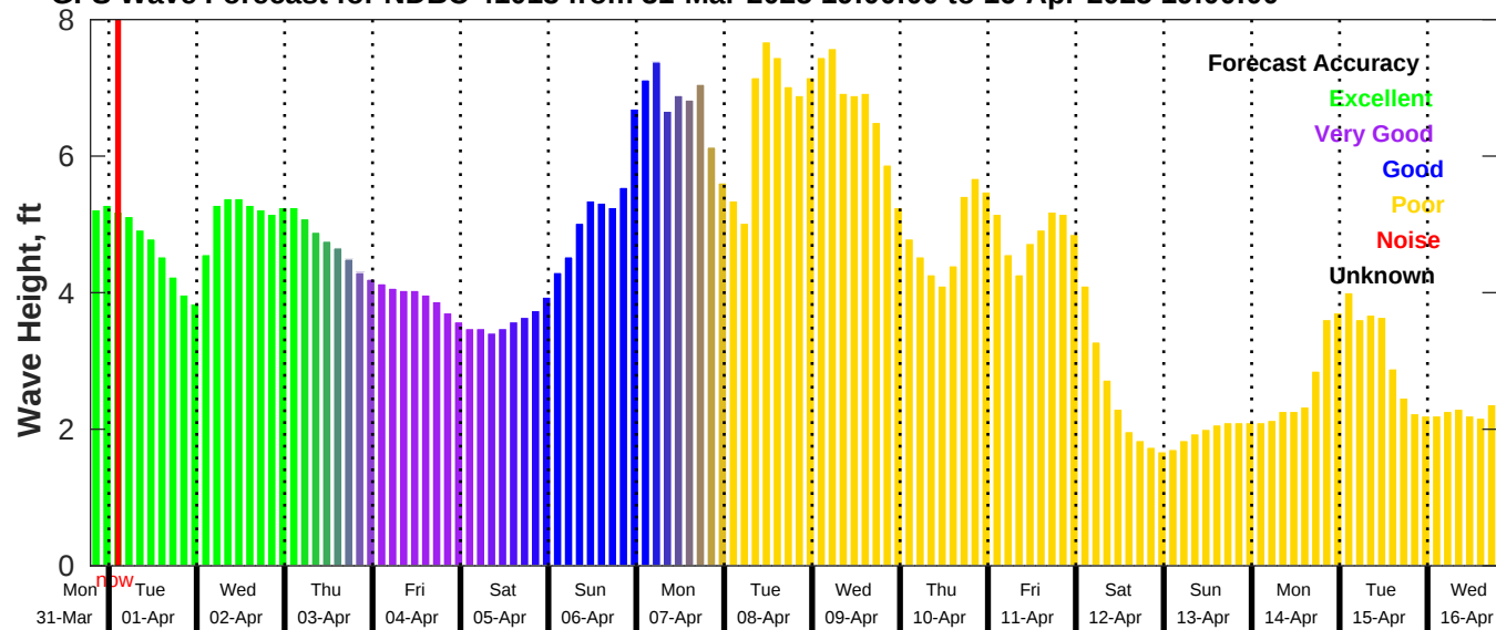
GFS Wave Forecast for NDBC 41013 from 31-Mar-2025 19:00:00 to 16-Apr-2025 19:00:00
