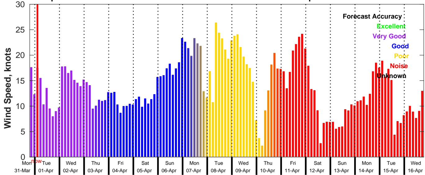
GFS Wind Speed Forecast for NDBC 41013 from 31-Mar-2025 19:00:00 to 16-Apr-2025 19:00:00
