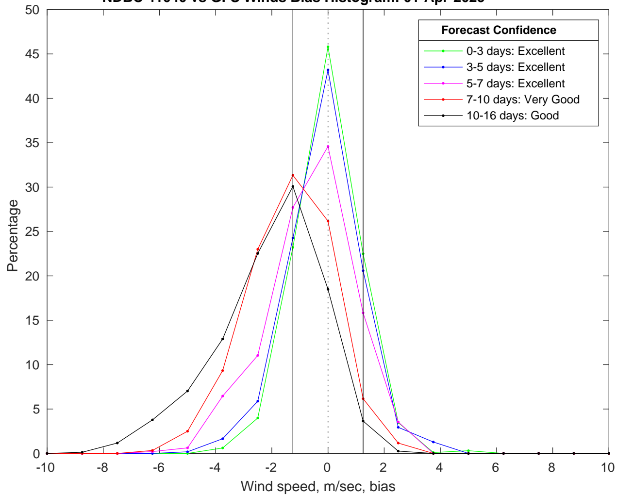
NDBC 41040 vs GFS Winds Bias Histogram: 01-Apr-2025
