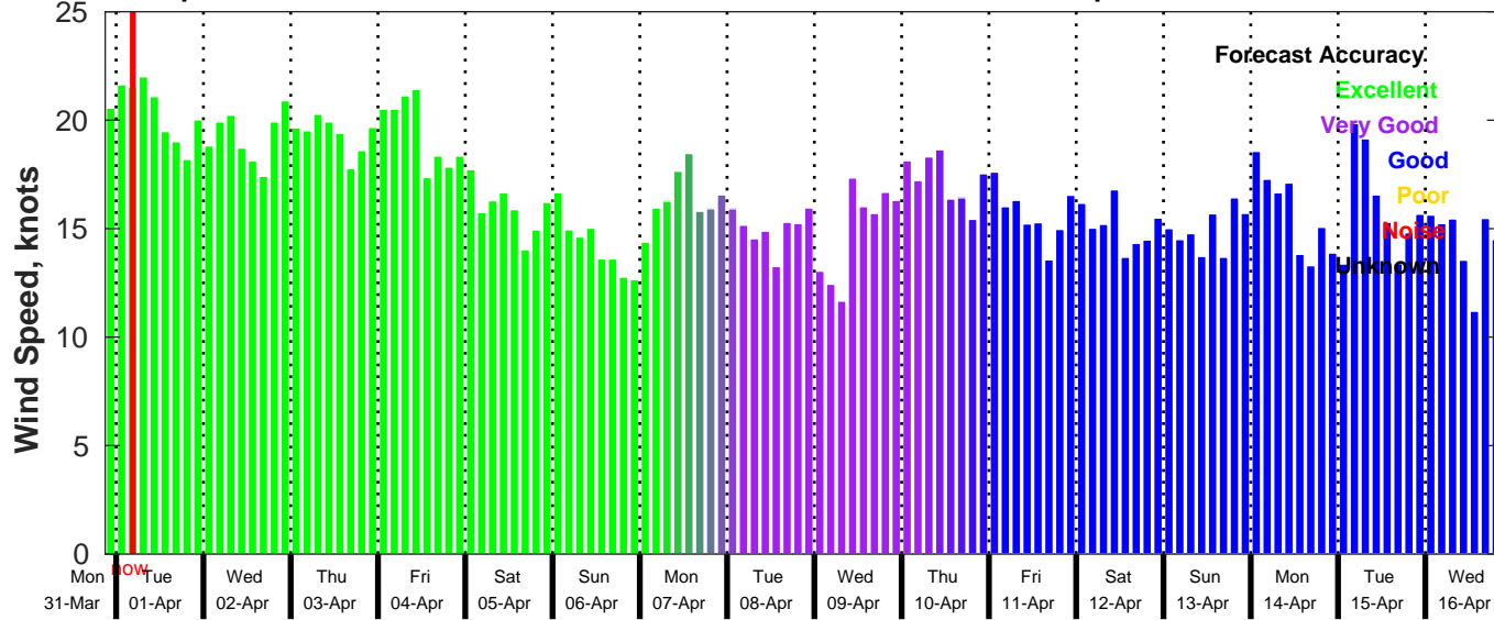
GFS Wind Speed Forecast for NDBC 41040 from 31-Mar-2025 21:00:00 to 16-Apr-2025 21:00:00
