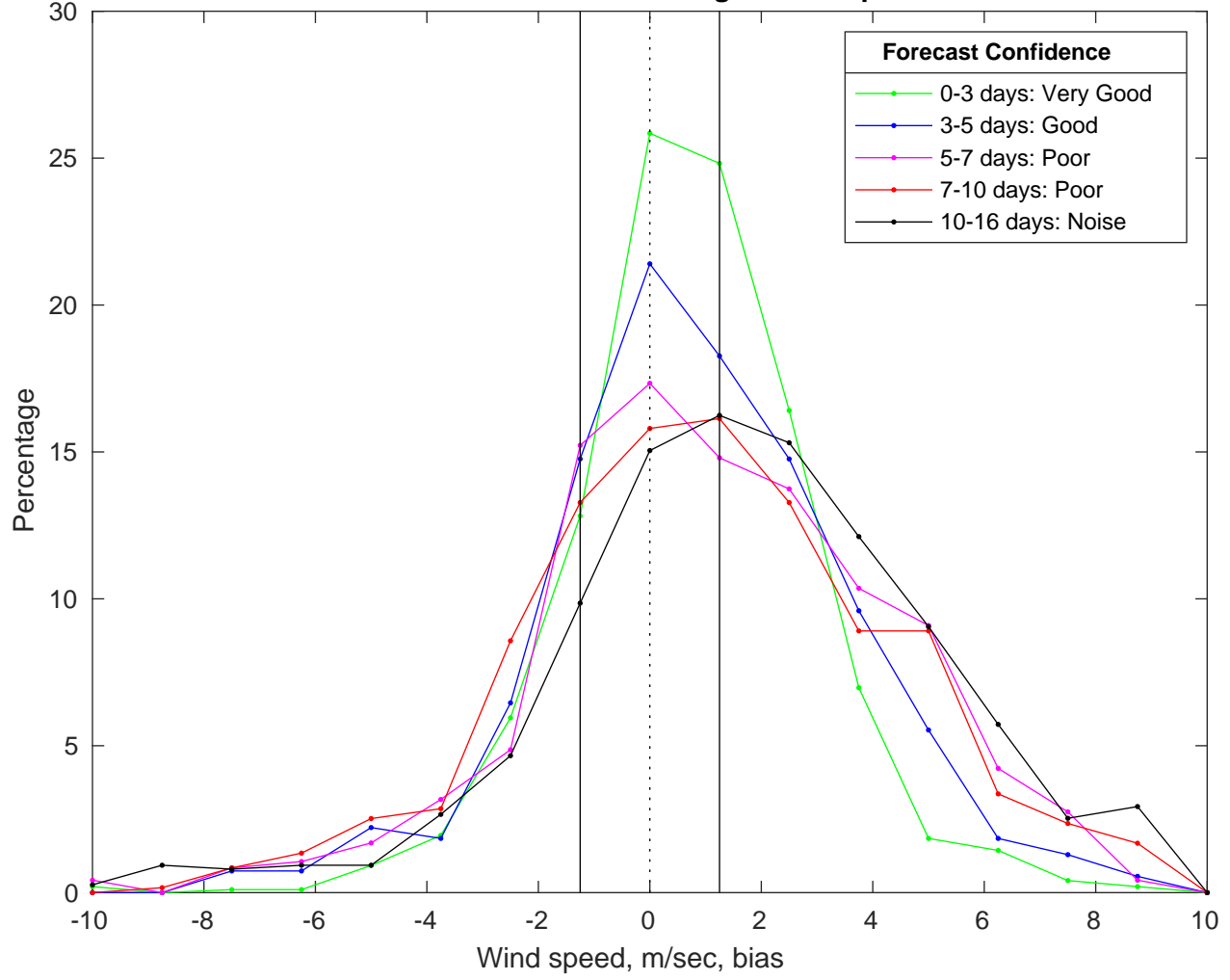
NDBC 42019 vs GFS Winds Bias Histogram: 01-Apr-2025
