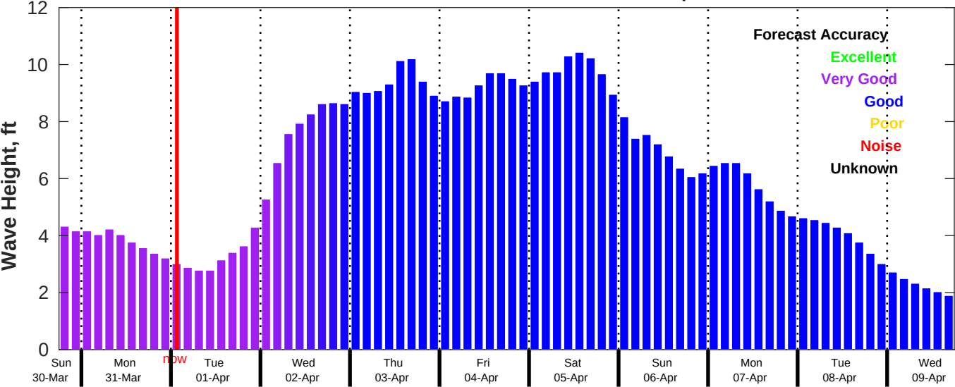
CMEMS Wave Forecast for NDBC 42019 from 30-Mar-2025 18:00:00 to 09-Apr-2025 18:00:00
