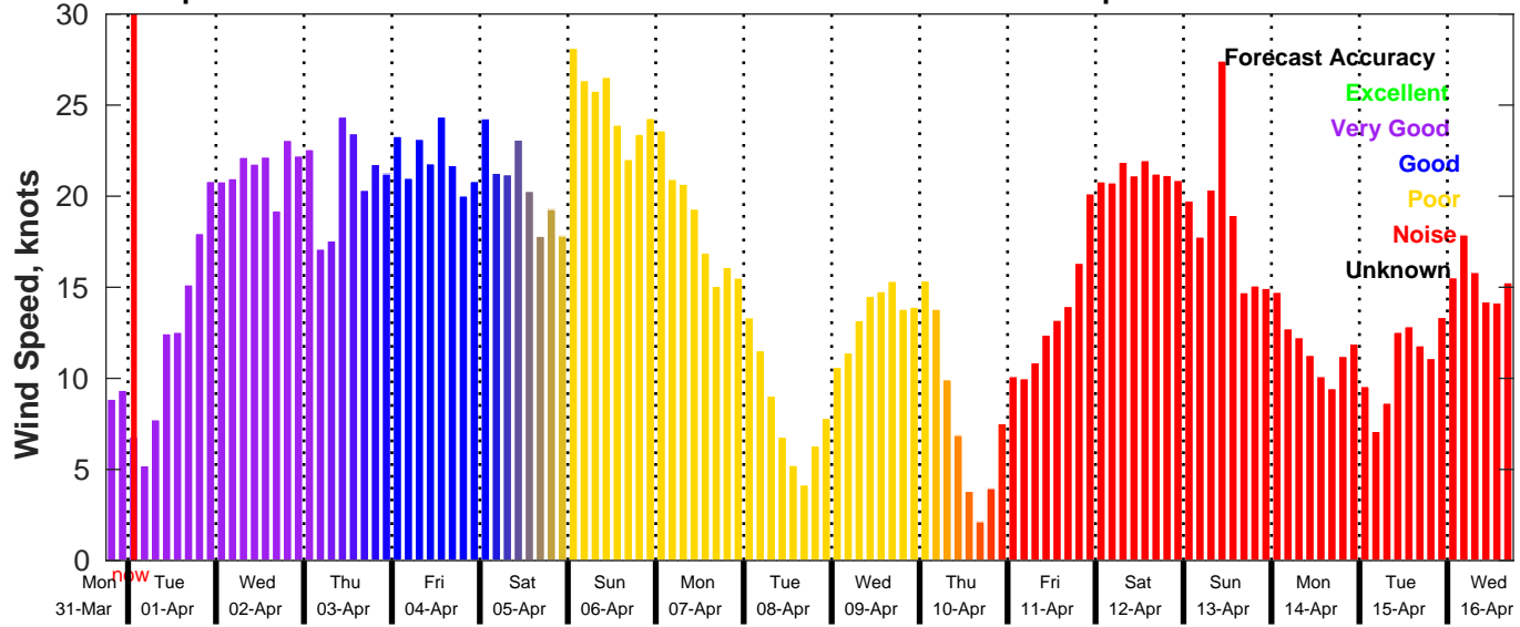
GFS Wind Speed Forecast for NDBC 42019 from 31-Mar-2025 18:00:00 to 16-Apr-2025 18:00:00
