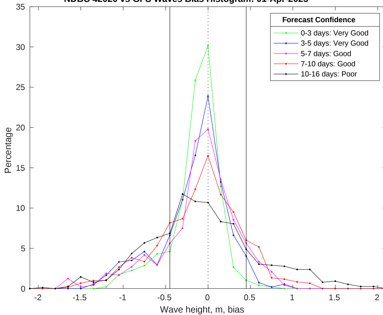
NDBC 42020 vs GFS Waves Bias Histogram: 01-Apr-2025
