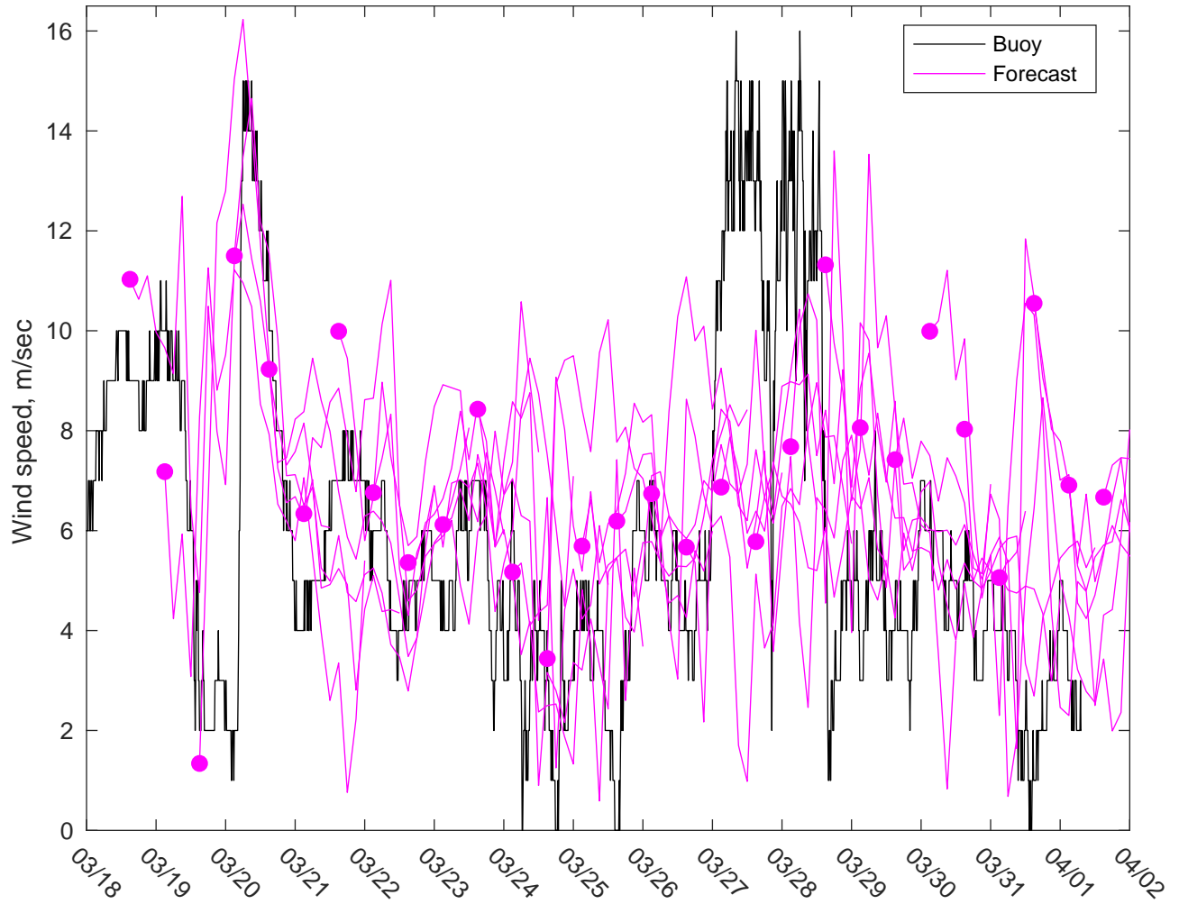
NDBC 42020 vs GFS Winds: 7 to 10 day forecast
