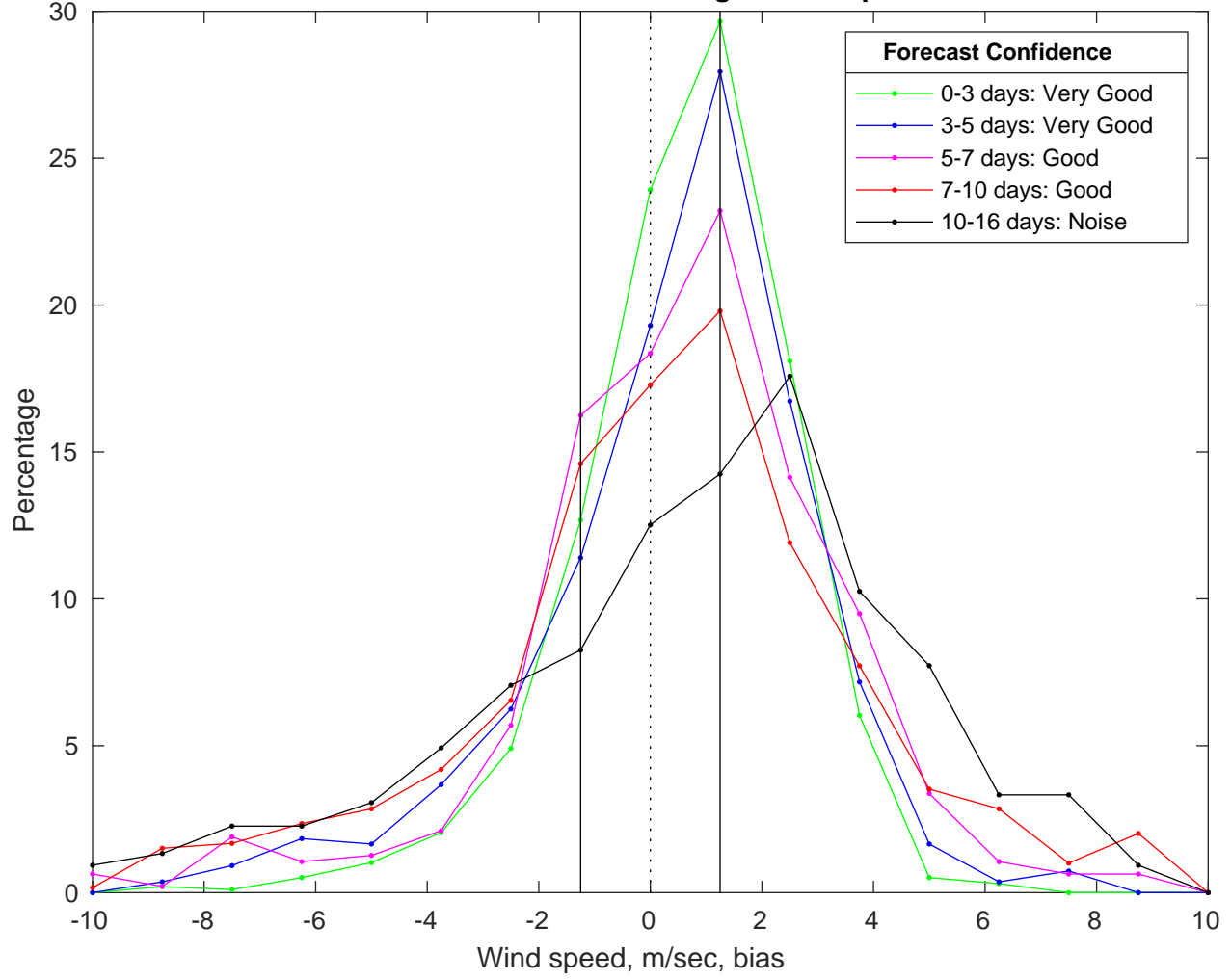
NDBC 42020 vs GFS Winds Bias Histogram: 01-Apr-2025
