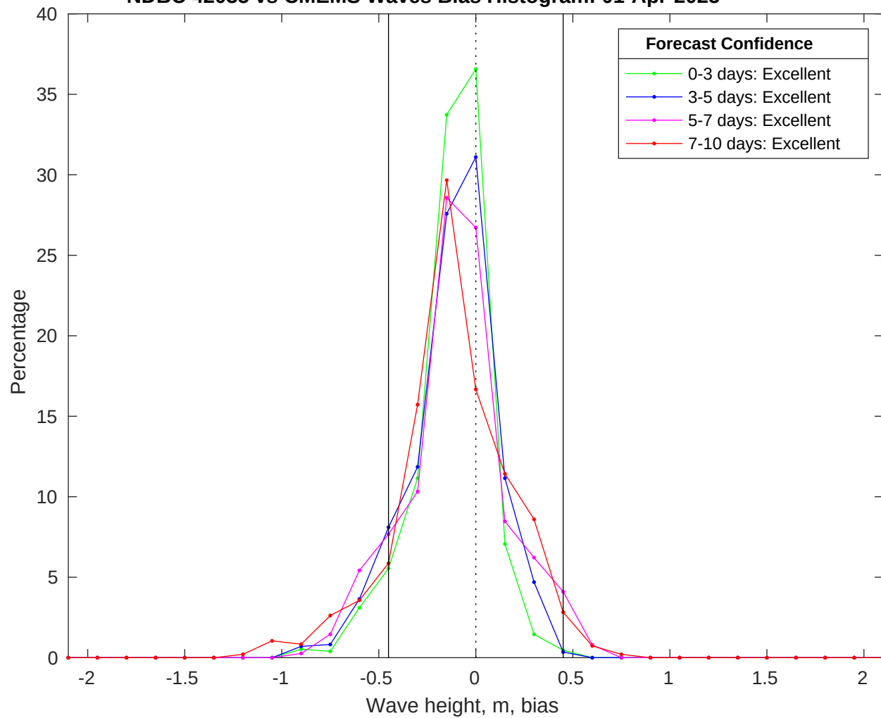
NDBC 42035 vs CMEMS Waves Bias Histogram: 01-Apr-2025
