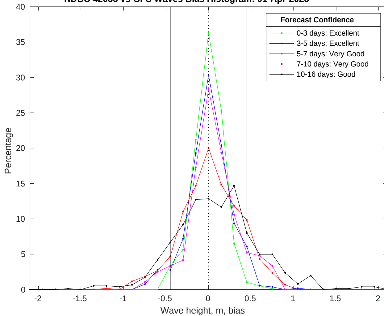
NDBC 42035 vs GFS Waves Bias Histogram: 01-Apr-2025
