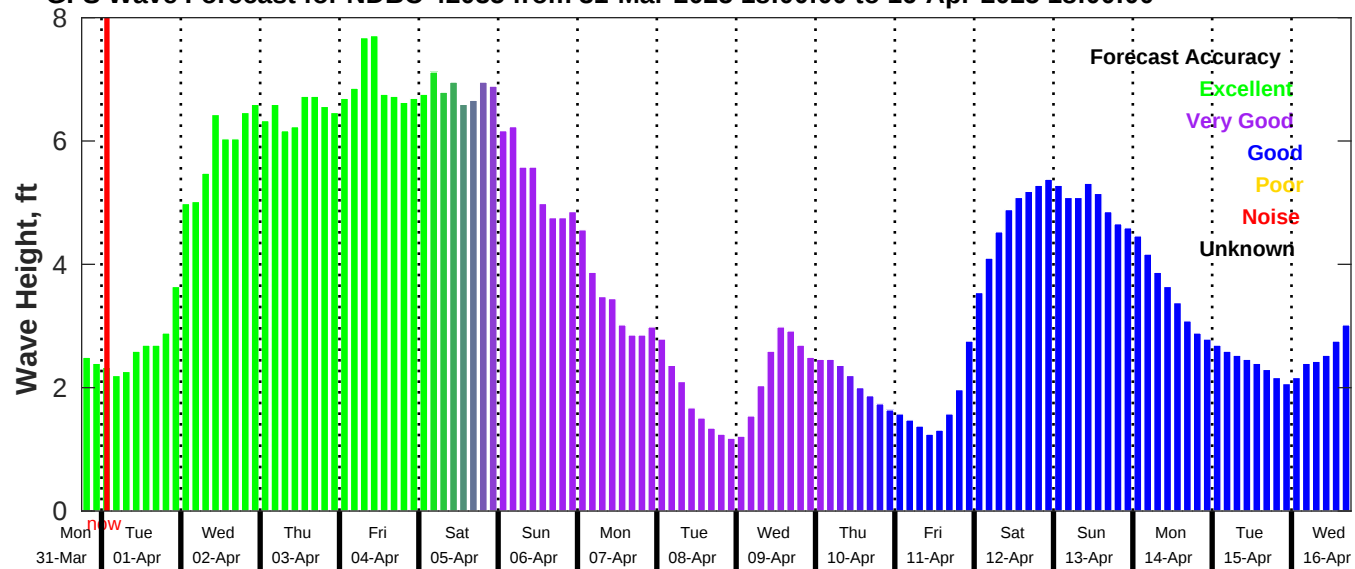
GFS Wave Forecast for NDBC 42035 from 31-Mar-2025 18:00:00 to 16-Apr-2025 18:00:00
