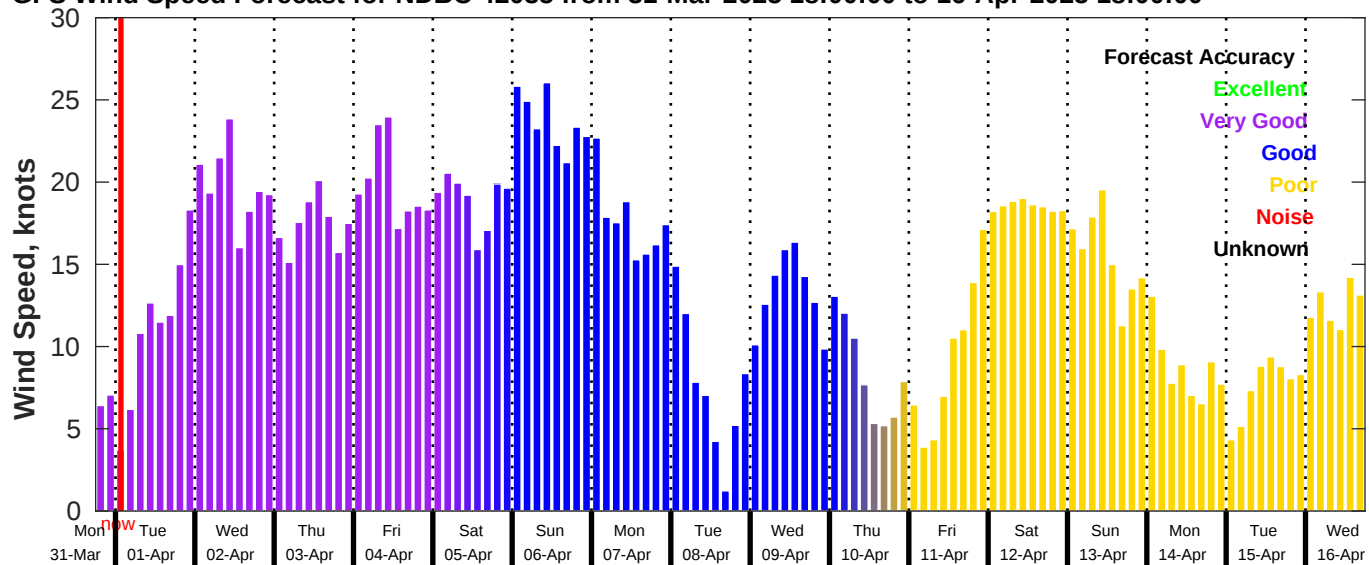
GFS Wind Speed Forecast for NDBC 42035 from 31-Mar-2025 18:00:00 to 16-Apr-2025 18:00:00
