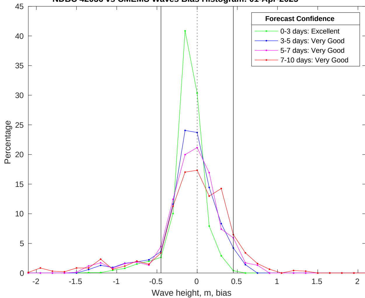
NDBC 42036 vs CMEMS Waves Bias Histogram: 01-Apr-2025
