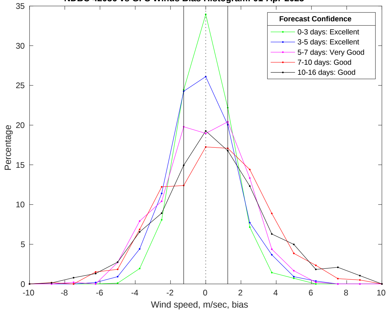
NDBC 42036 vs GFS Winds Bias Histogram: 01-Apr-2025
