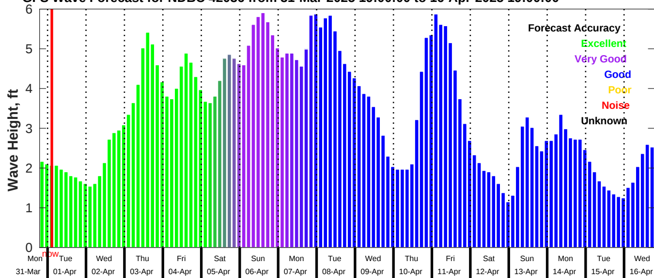
GFS Wave Forecast for NDBC 42036 from 31-Mar-2025 19:00:00 to 16-Apr-2025 19:00:00
