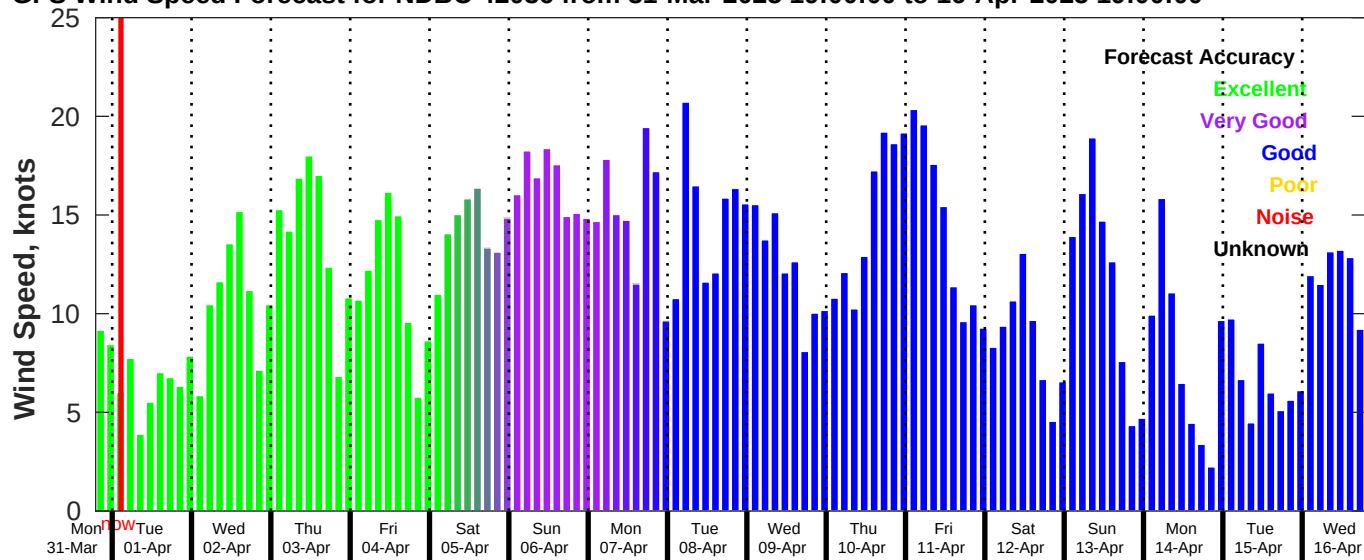
GFS Wind Speed Forecast for NDBC 42036 from 31-Mar-2025 19:00:00 to 16-Apr-2025 19:00:00
