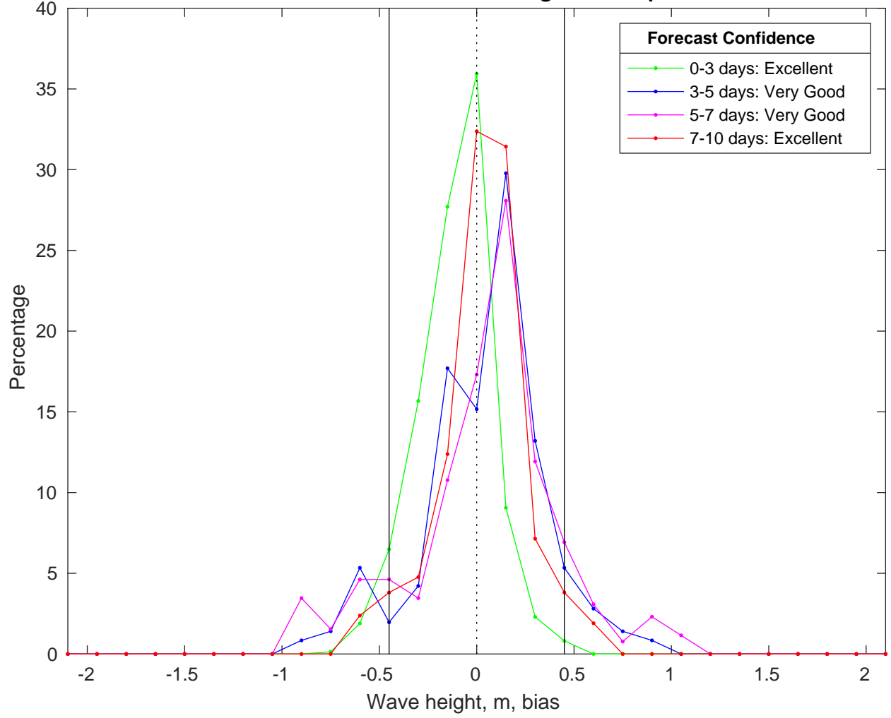
NDBC 42040 vs CMEMS Waves Bias Histogram: 01-Apr-2025
