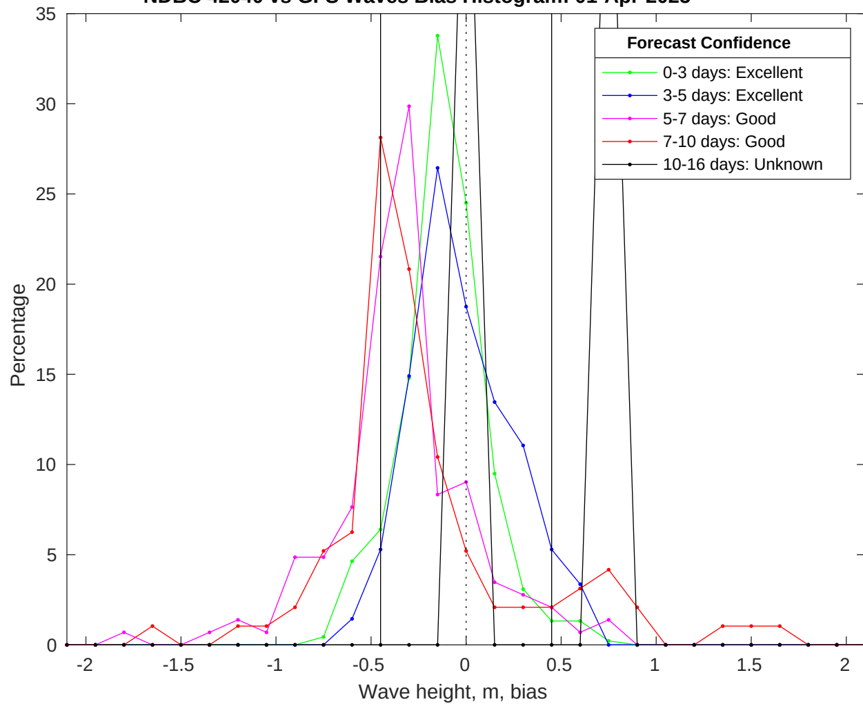
NDBC 42040 vs GFS Waves Bias Histogram: 01-Apr-2025
