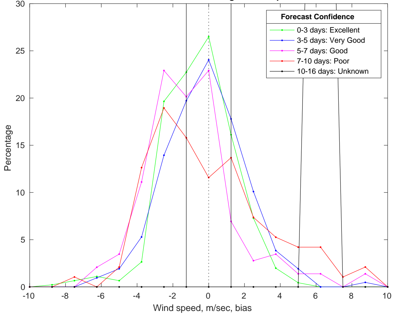
NDBC 42040 vs GFS Winds Bias Histogram: 01-Apr-2025
