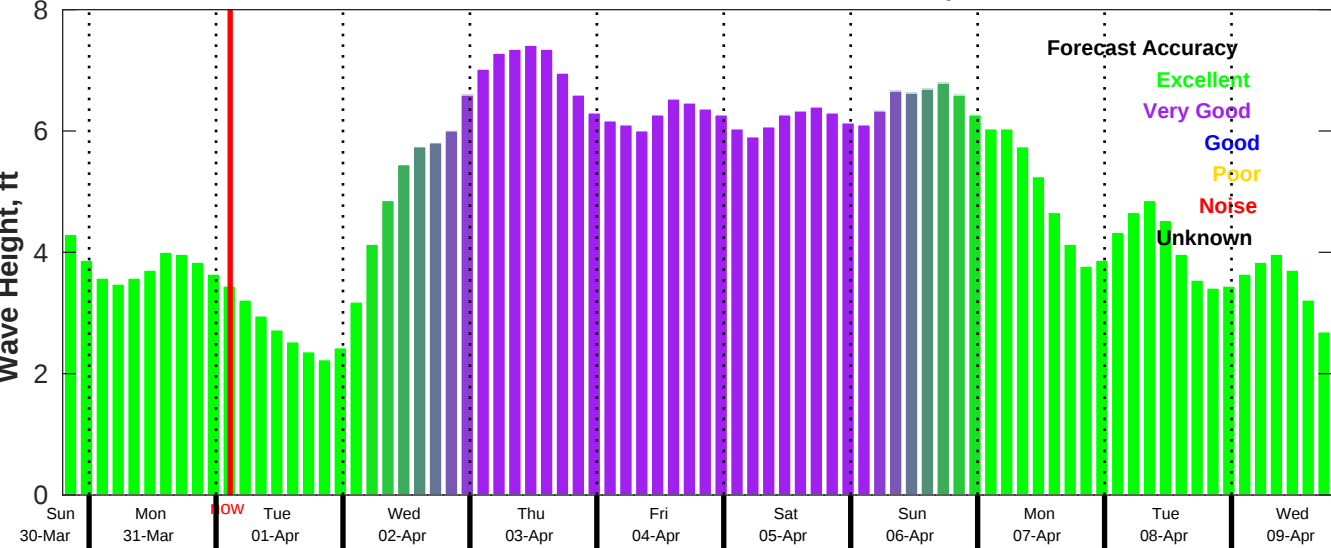
CMEMS Wave Forecast for NDBC 42040 from 30-Mar-2025 19:00:00 to 09-Apr-2025 19:00:00
