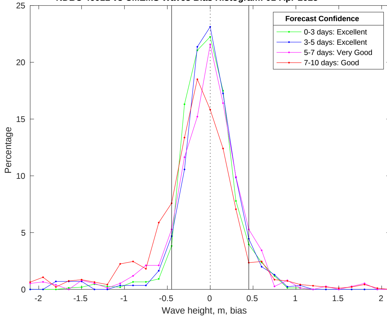
NDBC 46011 vs CMEMS Waves Bias Histogram: 01-Apr-2025
