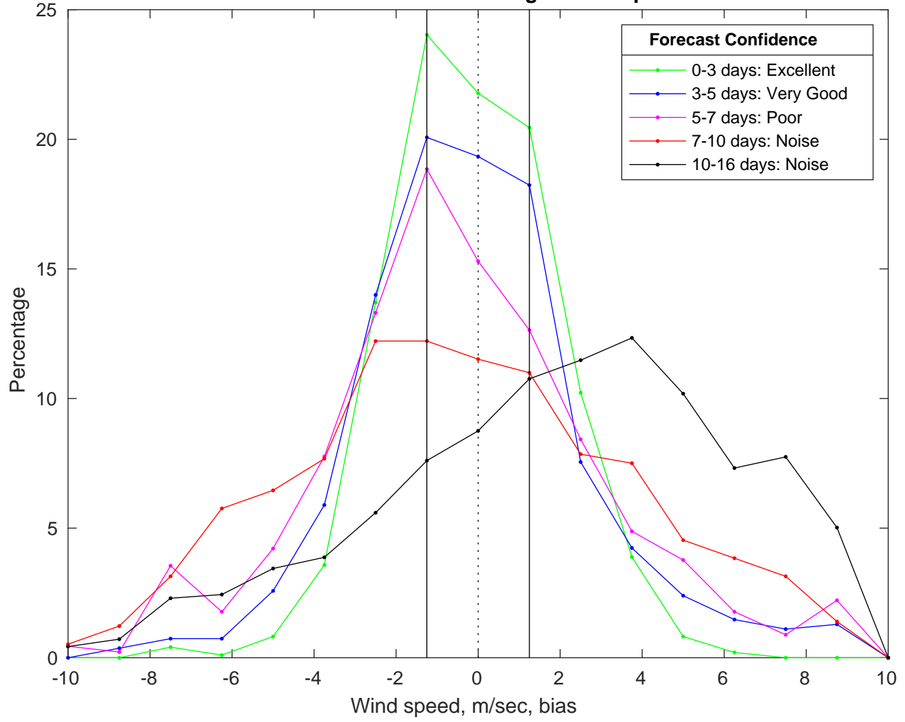
NDBC 46011 vs GFS Winds Bias Histogram: 01-Apr-2025
