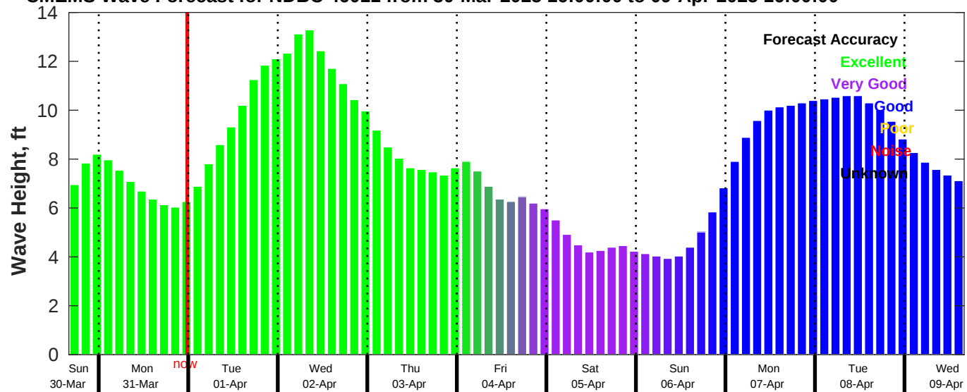
CMEMS Wave Forecast for NDBC 46011 from 30-Mar-2025 16:00:00 to 09-Apr-2025 16:00:00
