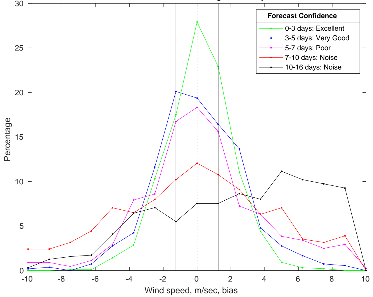
NDBC 46028 vs GFS Winds Bias Histogram: 01-Apr-2025
