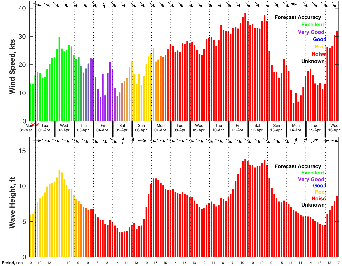
Wind & Wave Forecast for NDBC 46028 from 31-Mar-2025 16:00:00 to 16-Apr-2025 16:00:00
