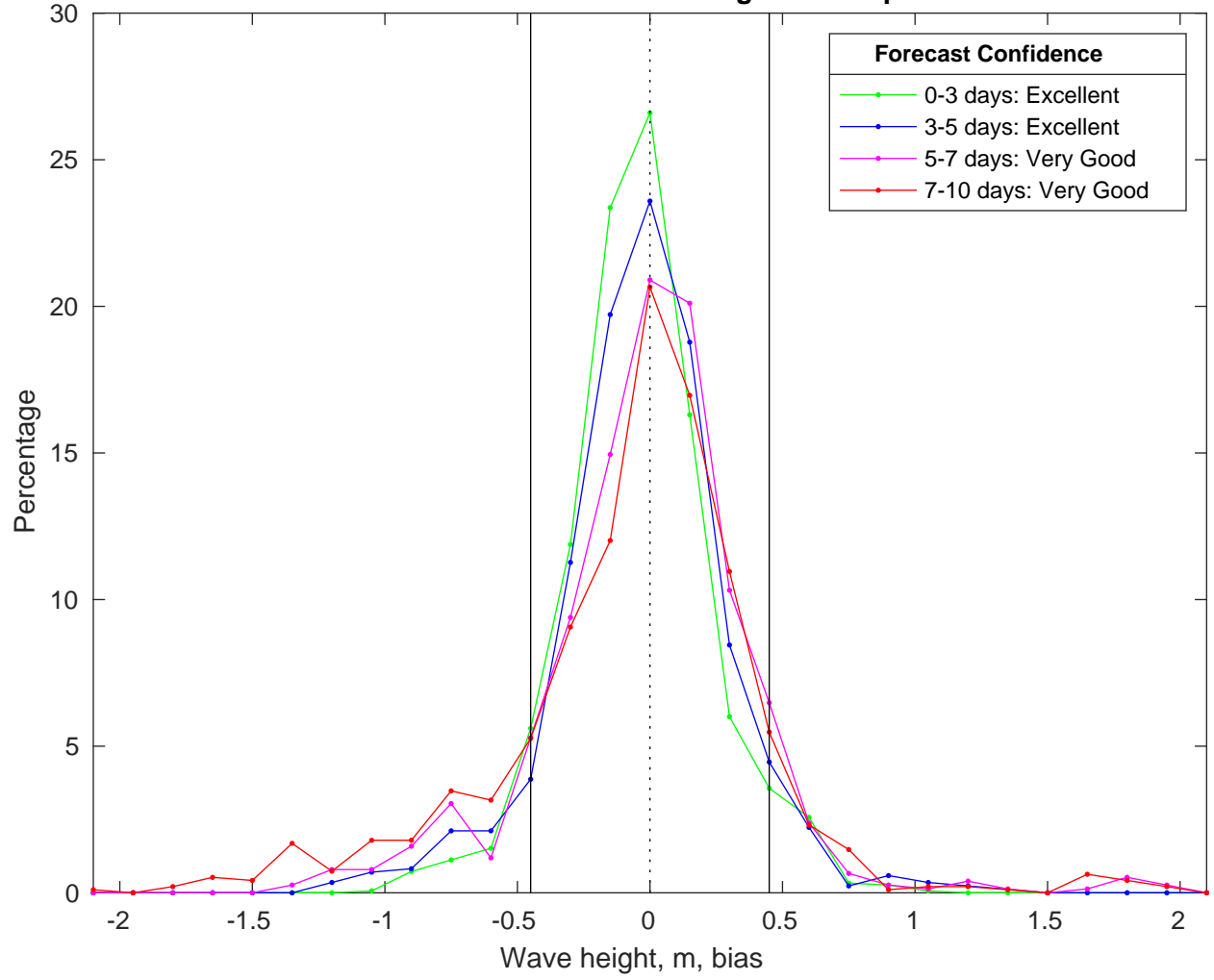
NDBC 46054 vs CMEMS Waves Bias Histogram: 01-Apr-2025
