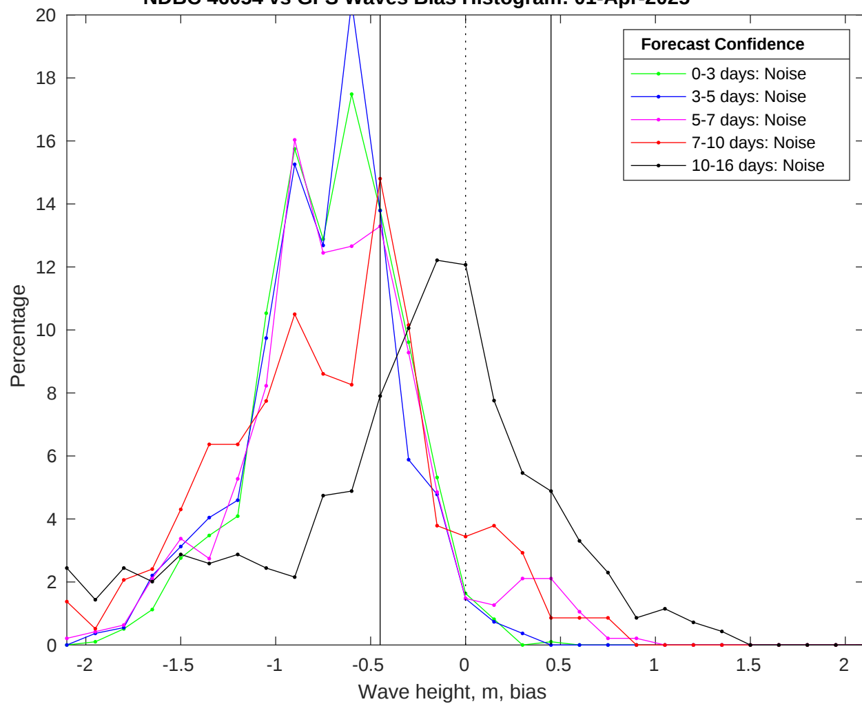
NDBC 46054 vs GFS Waves Bias Histogram: 01-Apr-2025
